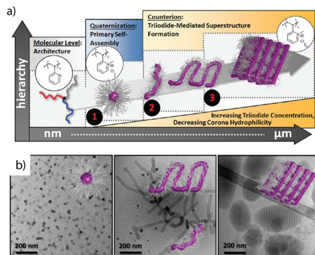
Fig. 16 Counterion-mediated structuring of \mu -(BVqT) +/I – miktoarm star terpolymers in water. (a) Hierarchical self-assembly mechanism and morphological evolution with iodine content. (b) Spherical micelles, worm-like micelles and axially stacked lamellae in ellipsoidal MCNs. Reprinted from ref. 299 with permission from American Chemical Society.
