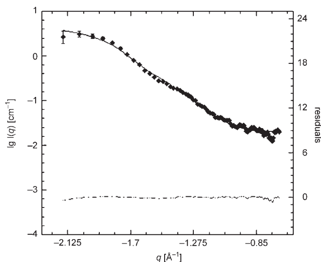
Figure 3. SANS curve of a 1-wt% aqueous solution of PAA 42 -b-PAAm 417 and P2MVP 42 -b-PEO 446 . Experimental data (♦), form factor fit (solid line) to a uniform, monodisperse oblate ellipsoid, and residuals (dotted line). S(q) and core-shell structure are not included in the fit.
